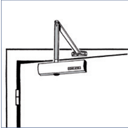
TS 2000 NV Door leaf installation/hinge side
