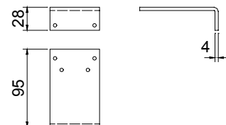
TS2000 PARALLEL ARM BRACKET
