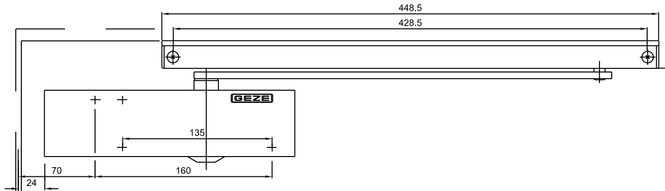
OPTION 1 - WITH SOFFIT ANGLE BRACKET
