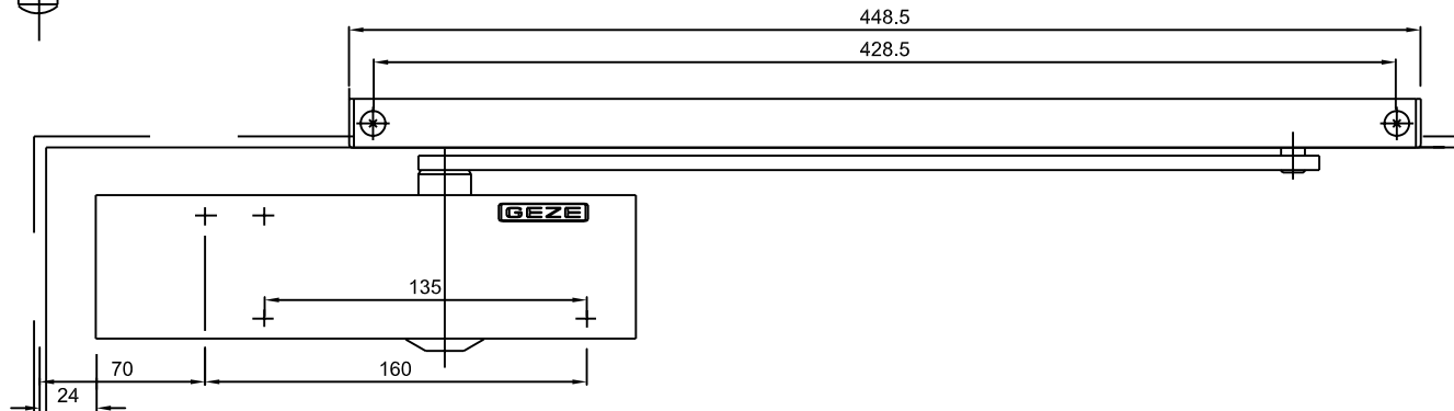
OPTION 2 - WITHOUT SOFFIT ANGLE BRACKET FOR FLUSH OVERPANEL OR MAX REVEAL 20mm
